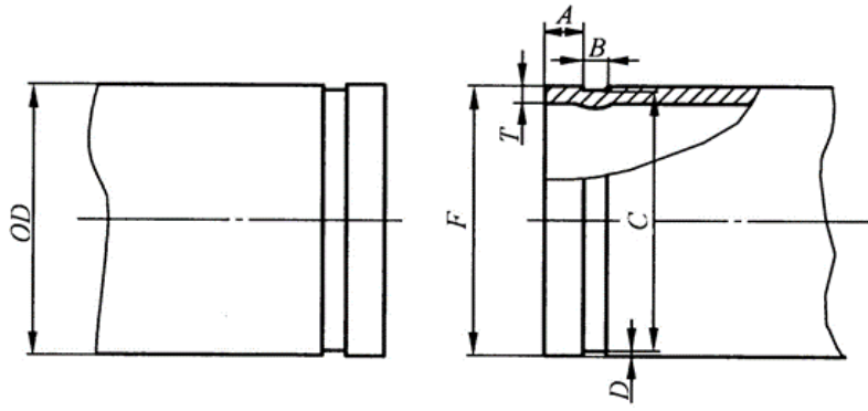
Dimensions and specifications of Rolling Groove end face
